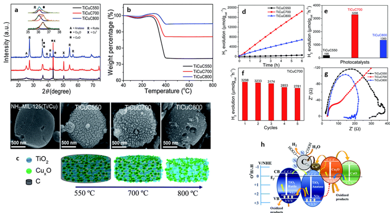
Fig. 7 (a) Powder X-ray diffraction patterns, (b) TGA in air, and (c) SEM images representative schematic diagrams of bi-MOF NH 2 -MIL-125(Ti/Cu) derived nanocomposites TiCuC550, TiCuC700 and TiCuC800 obtained at pyrolysis temperatures of 550, 700 and 800 C respectively. (d) Photocatalytic H 2 evolution performance of samples change with the reaction time; (e) comparison of photocatalytic H 2 evolution in μmol g cat -1 h -1 of TiCuC550 (black), TiCuC700 (red) and TiCuC800 (blue); (f) the recyclability test of the selected TiCuC700 nanocomposite and (g) EIS Nyquist plots of TiCuC550, TiCuC700, and TiCuC800 at the same potential in 0.5 M H 2 SO 4 . (h) the schematic illustration of the proposed mechanism of photocatalytic H 2 evolution over NH 2 -MIL-125(Ti/Cu) derived multi-heterojunction TiCuC700 under UV-vis light MIL-125(Ti/Cu). 57
