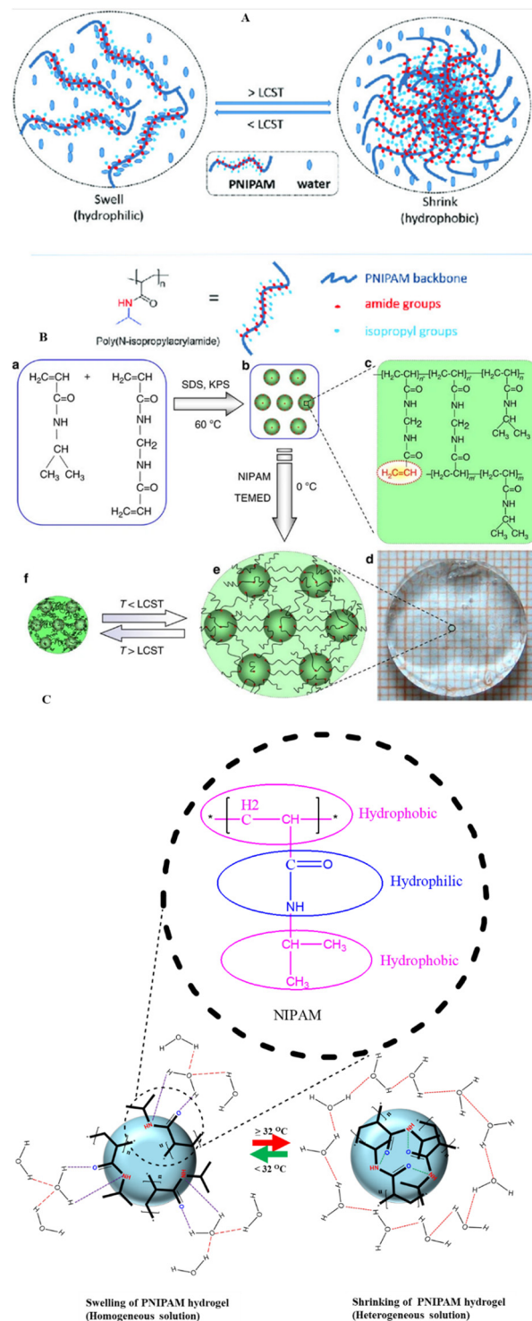
Fig. 7 (A) Schematic view of temperature dependent sol gel transition of PNIPAM based hydrogel. (B). Chemical structures of PNIPAM and N,N -methylene bis acrylamide (MBA) (a), copolymer of NIPAM and MBA synthesized by precipitation polymerization (b), Structure of the synthesized activated NIPAM based nano gel (c), optical image of the hydrogel constructed from NIPAM and activated nanogel at low temperature (d), schematic of the copolymer hydrogel at temperature < LCST (e) and > LCST (f). (C) Diagrammatic illustration of swelling (hydration) and shrinkage (precipitate formation) of PNIPAM hydrogel. (A) is adapted from ref. 186 and (B) from ref. 187 (with permission of the publisher copyright Royal Society of Chemistry 2023).
