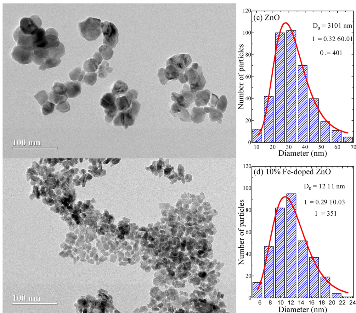
Fig. 5 (a) TEM for the undoped and (b) Fe-doped ZnO nanoparticles, with their corresponding particle size histograms (c) undoped and (d) Fe-doped ZnO. In panels (c and d) N means the number of counted particles. The solid lines represent the lognormal fit to each distribution.
