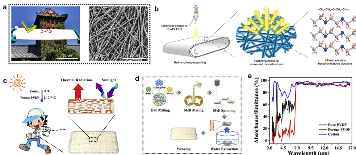
Fig. 2 (a) The photo (left) and SEM image of disordered nanofibers (right) of the electrospun PEO nanofiber-based membrane. (b) Schematic illustration of roll-to-roll electrospinning fabrication process (left) for micro- and nano-structured film (middle) schematic diagram of PEO molecular chain bond vibration (right). Reproduced with permission from ref. 52. Copyright, 2021 Nature Publishing Group. Schematic illustration of (c) porous PVDF textile, and (d) manufacturing process of the PVDF fibre. (e) The near-infrared and mid-infrared absorbance/emittance curves of porous PVDF, pure PVDF and cotton. Reproduced with permission from ref. 57. Copyright, 2020 Elsevier.
