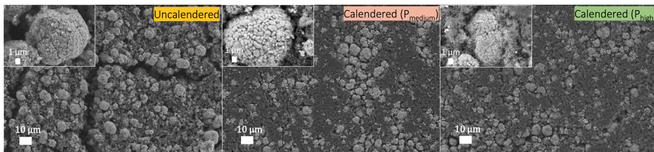
Fig. 7 SEM surface analysis of lignin/water cathode coatings with a similar mass loading ( 7.4 \pm 0.3 \text{ mg cm}^{-2} ) which was uncalendered, calendered at medium pressure using a 60 μm calendering gap ( P_{\text{medium}} ), or calendered at high pressure using a 45 μm calendering gap ( P_{\text{high}} ) (magnitude: 1000 \times ). The NMC111 particles are shown in the top right corner (magnitude: 10 000 \times ). The rate capability of these cathodes is shown in Fig. 10b.
