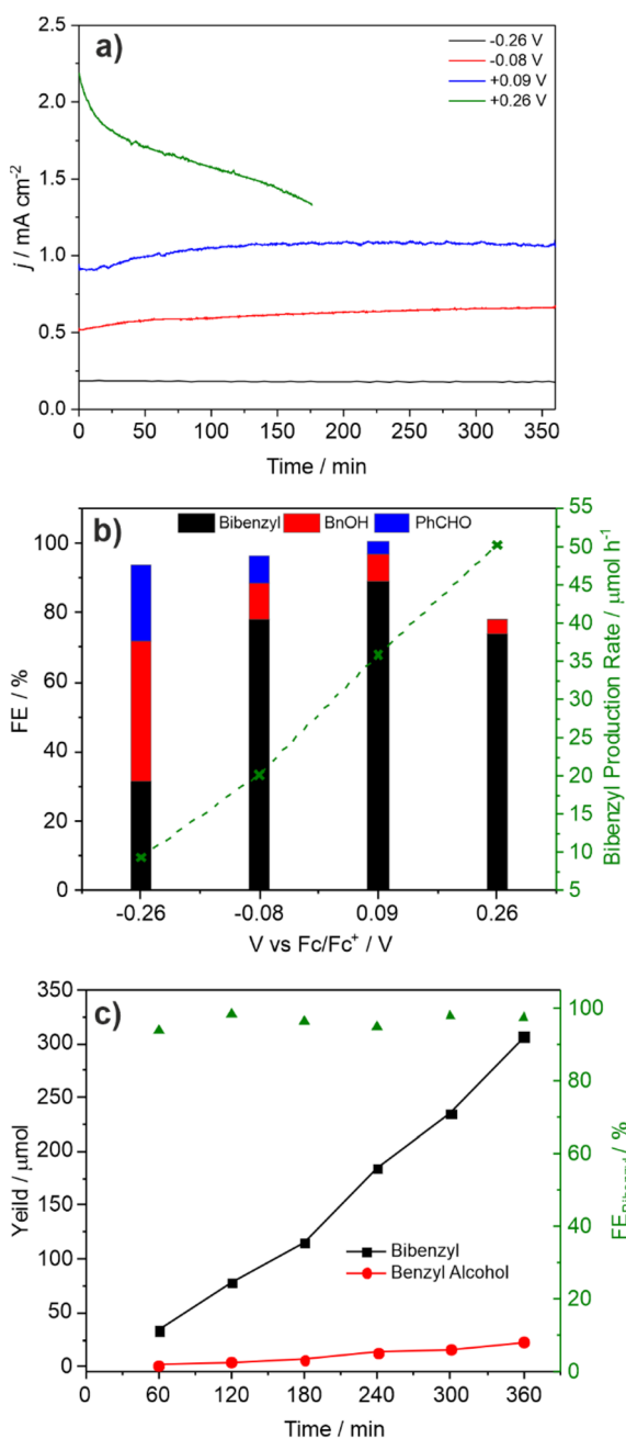
Fig. 3 (a) CPE of 1 M PAA with 0.05 equiv. \text{Et}_3\text{N} at -0.26 (black), -0.08 (red), +0.09 (blue) and +0.26 V (green) vs. \text{Fc}/\text{Fc}^+ ; (b) faradaic efficiencies for bibenzyl (black), benzyl alcohol (red) and benzaldehyde (blue) as a function of electrolysis potential; (c) time-dependent bibenzyl (black) and benzyl alcohol (red) formation at +0.09 V vs. \text{Fc}/\text{Fc}^+ of 1 M PAA with 0.05 equiv. \text{Et}_3\text{N} . Overall faradaic efficiency for bibenzyl is given in green.
