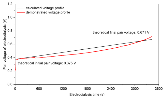
Fig. 4 The voltage profiles of one electrodiolysis pair along with electrodiolysis time for \text{NO}_3^- concentration. A single electrodiolysis pair is constructed by the configuration of “CEM | diluate | AEM | concentrate” in which the CEM and the AEM are FKA-PK-130 and FAA-PK-130, respectively, both from Fuma-Tech; and the diluate and the concentrate are 7.14 mM \text{KNO}_3 (100 ppm \text{NO}_3^- -N) and 2 M \text{KNO}_3 (28 000 ppm \text{NO}_3^- -N), respectively. The key experimental conditions include: 5 \text{cm}^2 as the effective pair area, 1 \text{mA cm}^{-2} as the electrodiolysis current density, 10 \text{cm s}^{-1} as the nominal fluid velocity for all channels (60 \text{mL min}^{-1} ), 0.5 mm as the distance between CEM and AEM in the electrodiolysis pair, and 75% as the designed \text{NO}_3^- removal (3444 seconds). Note that the applied current density for ED is subject to the threshold set by the “limiting current density” calculated by the Rosenberg and Tirrell equation, 41 and the obtained limiting current density is 4.62 and 1.19 \text{mA cm}^{-2} at the initial (7.14 mM) and the final diluate concentration (1.79 mM), respectively, under our experimental conditions.
