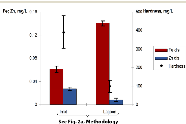
Fig. 7 Metals and water hardness profile during dry weather Fe dis is 0.14 mg L -1 in the lagoon, comprising almost 50% of its total form (Fe tot is 0.29 mg L -1 ).
