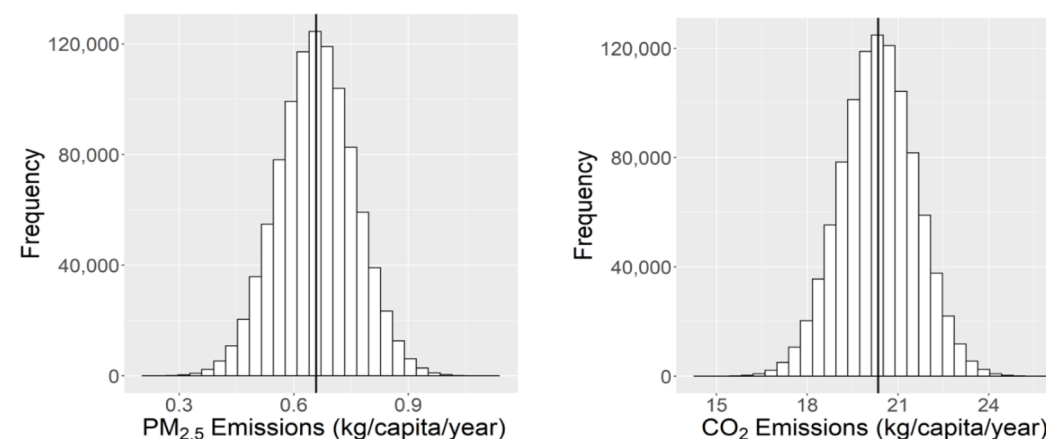
Fig. 2 Particulate matter ( \text{PM}_{2.5} , left) and carbon dioxide ( \text{CO}_2 , right) annual emission estimate distribution from Monte Carlo samplings for (a) the Xalapán region of Jalapa, (b) the city of Jutiapa, and (c) Guatemala city.
