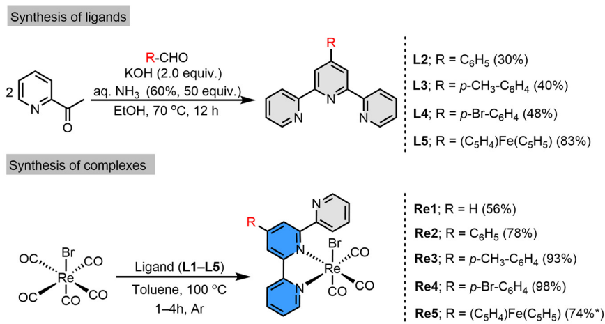
Scheme 1 Synthesis of terpyridine ligands (L2–5) and fac - \text{Re}(\text{i})(\text{L})(\text{CO})_3\text{Br} complexes ( Re1–5 ), where L = L1–5. * Re5 contains toluene (~0.5 molecules, calculated from ^1\text{H} NMR) as a solvent of crystallisation.
