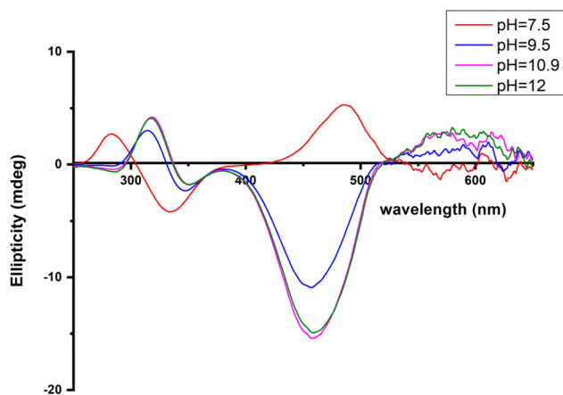
Fig. 6 Circular dichroism spectra of the solutions of Cu(II) and R1P ( \text{Cu(II)} : \text{R1P} = 1 : 1.2 ), recorded at the indicated pH values.
