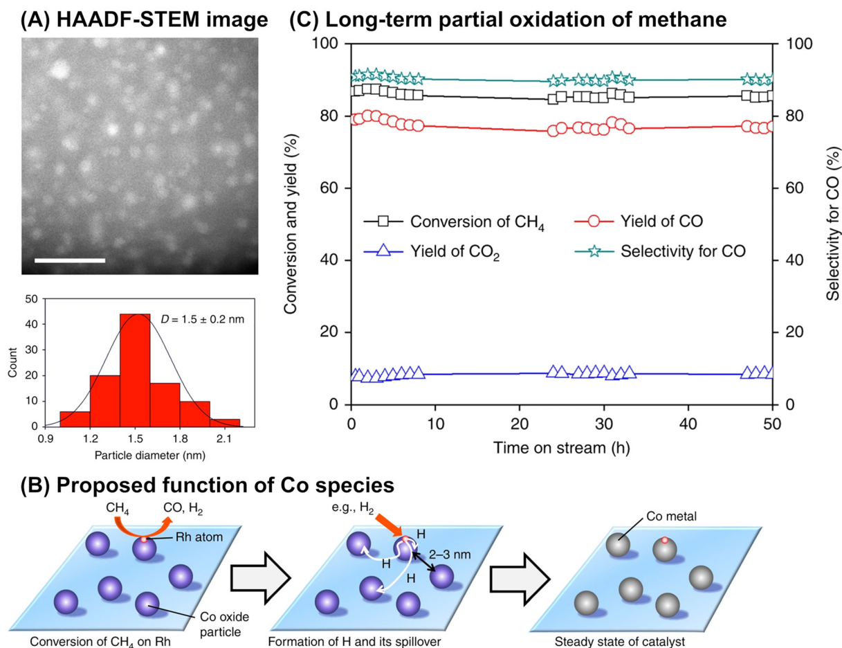
Fig. 19 (A) HAADF-STEM image of 0.005 wt% Rh-3 wt% Co/MOR catalyst, (B) proposed function of Co species for reducing Rh species via hydrogen spillover, and (C) long-term partial oxidation of methane over the Rh-Co/MOR catalyst. Reaction conditions: \text{CH}_4/\text{O}_2/\text{N}_2 = 3.33/1.67/95 ; \text{SV} = 1.2 \times 10^6 \text{ mL h}^{-1} \text{ g}_{\text{cat}}^{-1} ; 923 K; 0.1 MPa. Reproduced from ref. 79 with permission from Springer Nature, copyright 2018.
