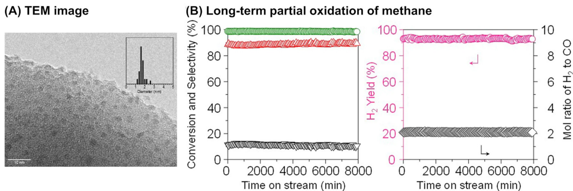
Fig. 18 (A) TEM image of 5 wt% Ni/MOR catalyst and (B) long-term partial oxidation of methane over the Ni/MOR catalyst. Reaction conditions: \text{CH}_4/\text{O}_2/\text{Ar} = 0.06/0.03/0.91 atm; \text{SV} = 3.0 \times 10^4 \text{ mL h}^{-1} \text{ g}_{\text{cat}}^{-1} ; 973 K. Reproduced from ref. 77 with permission from Springer Nature, copyright 2020.
