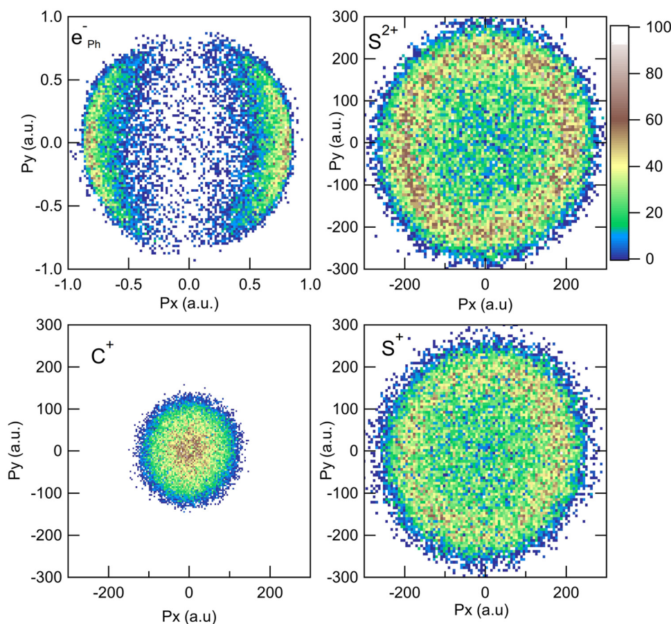
Fig. 1 Momentum distributions recorded in the laboratory frame for the \text{S}^{2+} + \text{C}^{+} + \text{S}^{+} + \text{e}_{\text{ph}}^{-} PE3PICO channel after core S 1s photoionization in \text{CS}_2 .
