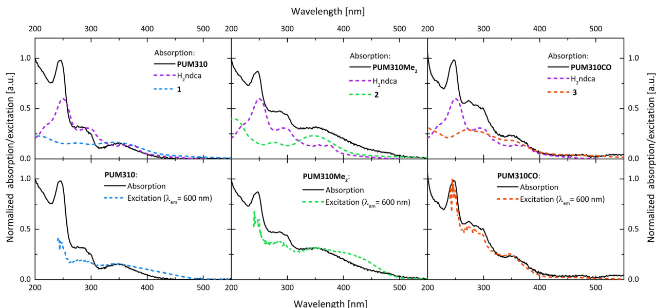
Fig. 7 Top: Comparison between the absorption spectra of PUM310 , PUM310Me 2 , PUM310CO (continuous black lines), \text{H}_2\text{ndca} (dashed violet lines), 1 (dashed blue line), 2 (dashed green line) and 3 (dashed orange line). Bottom: Comparison between the absorption spectra of PUM310 , PUM310Me 2 , and PUM310CO and the corresponding excitation spectra obtained collecting the acceptor emission at 600 nm.
