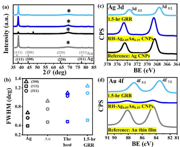
Fig. 4 Characterization of the host \text{RH-Ag}_{0.85}\text{Au}_{0.15} CNPs and the \text{RH-Ag: Au} m-CNPs (produced by the 1.5 h-GRR of the host at T_{\text{AL}} = 20 nm) with (a) XRD and (c) and (d) XPS. (b) Plot of the full width of half maximum (FWHM) of the (111), (200) and (311) facets measured in (a). (a) The peaks marked with asterisks are assigned to the silicon wafers on which the CNPs are deposited. XPS: (c) Ag 3d; (d) Au 4f. Black and grey symbols: RH-Ag CNPs and Au thin films, respectively (as references); blue symbols: the host; cyan symbols: RH-Ag: Au m-CNPs.
