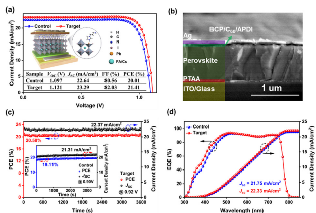
Fig. 3 (a) J - V curve of PSCs and the illustration of device structure based on ADPI modification, (b) cross-sectional SEM image of PSC, (c) stabilized power output at the maximum power point under AM 1.5G and (d) EQE for the control and target devices.
