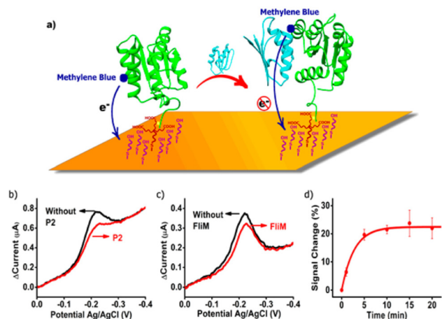
Fig. 3 (a) Figure showing the first reagentless protein-based electrochemical biosensor. Electrochemical response occurs when a target protein binds to the surface tethered protein recognition element, reducing the efficacy with which the attached reporter transfers electrons to the electrode surface when interrogated using a voltammetric technique. (b and c) Alteration in voltammetric response when the sensor was measured in a solution containing its binding partners (CheA-P2 or FliM). Figure reproduced from ref. 15, with permission from American Chemical Society, Copyright © 2017.
