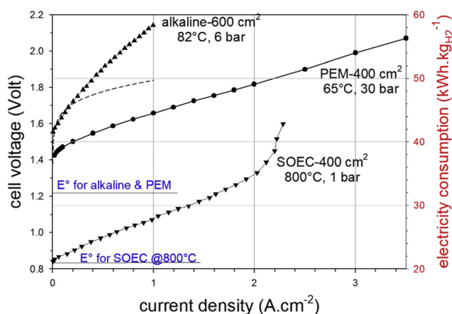
Fig. 4 Comparison of alkaline, PEM, and solid oxide electrolyzer cell (SOEC) technologies for electrolysis of water as a function of electricity consumption (current and voltage). 31 The indicative temperatures and pressures for each technology are a general representative of their operating conditions.
