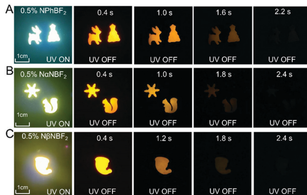
Fig. 2 Photographs of (A) NPhBF 2 –MeOBP-0.5%, (B) N \alpha NBF 2 –MeOBP-0.5% and (C) N \beta NBF 2 –MeOBP-0.5% afterglow materials under 365 nm UV light and after removal of the UV light.
