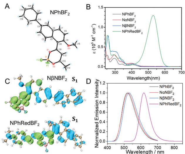
Fig. 1 (A) Single crystal structure of NPhBF 2 . (B) UV-vis spectra of naphthalene-containing BF 2 bdk in dichloromethane solutions. (C) TD-DFT calculated results of N \beta NBF 2 and NPhRedBF 2 S 1 states. Blue and green isosurfaces correspond to hole and electron distributions, respectively. TD-DFT calculations were performed in the ORCA 4.2.1 program with the B3LYP functional and def2-TZVP(-f) basis set. (D) Steady-state emission spectra of naphthalene-containing BF 2 bdk in dichloromethane solutions.
