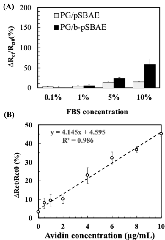
Fig. 8 (A) R_{ct} change [ \Delta R_{ct}/R_{ct0} (%)] on PG/pSBAE and PG/b-pSBAE ( 8/30 \text{ mg mL}^{-1} ) modified ITO after incubation in FBS solutions at different concentrations for 2 hours. (B) R_{ct} change [ \Delta R_{ct}/R_{ct0} (%)] of PG/b-pSBAE ( 8/30 \text{ mg mL}^{-1} ) coated ITO after immersion in 1% FBS containing different amounts of avidin.
