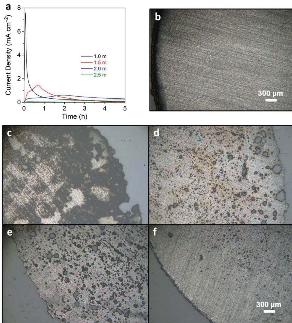
Fig. 1 (a) Chronoamperometry curves with an imposed potential of 4.5 V vs. \text{Li/Li}^+ for 5 h of aluminum current collectors when contacting 1.0, 1.5, 2.0, and 2.5 m LiTFSI in MPN electrolytes. Optical micrographs of (b) pristine aluminum, (c) 1.0, (d) 1.5, (e) 2.0, and (f) 2.5 m concentration after corrosion tests.
