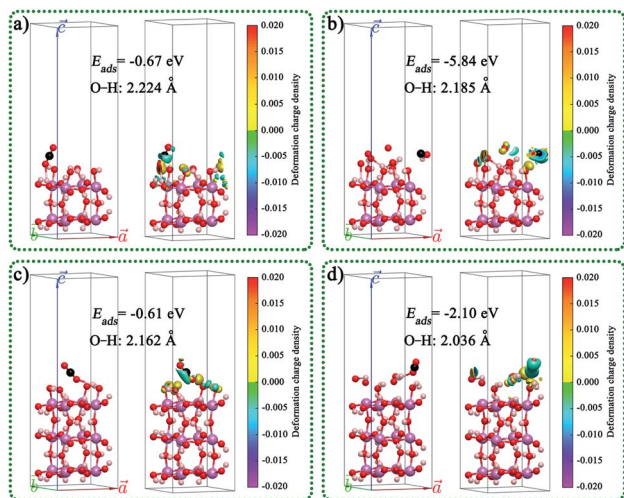
Fig. 7 CO 2 adsorbed on the (001) surface of In(OH) 3 with different section thicknesses, exposed atoms, and adsorption sites: (a) In 8 CO 26 H 24 , (b) In 8 CO 30 H 28 , (c) In 12 CO 38 H 36 , and (d) In 12 CO 40 H 40 .
