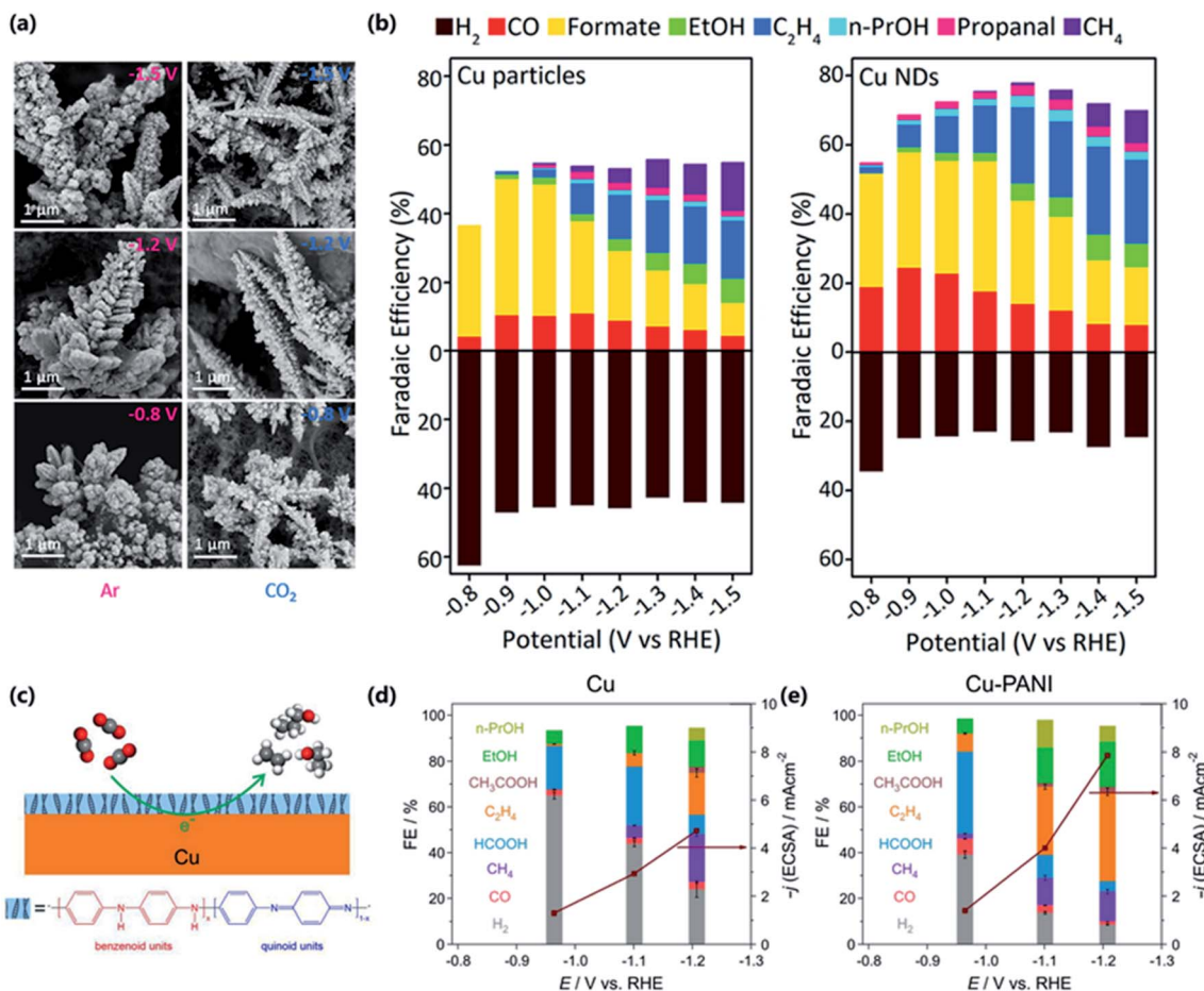
Fig. 7 (a) SEM images of Cu NDs at specific applied potentials after potentiostatic electrolysis for 20 min. (b) Faradaic efficiencies for the \text{CO}_2\text{RR} of the Cu particles (left) and the Cu NDs (right). Adapted with permission. 123 Copyright 2020, American Chemical Society. (c) Schematic diagram of the \text{CO}_2\text{RR} occurring at the Cu/PANI interface. (d) FE for every product and ECSA-normalized current density for the Cu. (e) FE for every product and ECSA-normalized current density for the Cu/PANI. Adapted with permission. 125 Copyright 2020, American Chemical Society.
