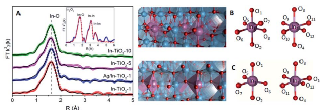
Fig. 3 (A) FT k 2 \chi(k) EXAFS spectra (spheres) of TiO 2-x samples and corresponding fit (black lines). The inset shows the extended fit for In 2 O 3 reference. The scale is uncorrected for the phase shift. Models of (B) stoichiometry and (C) vacancy structures. In the case of E In 1 Ti 1-x O 2-y ; In1: close to O V , In2: opposite to O V . Atom colours: Ti (blue), O (red), In (purple).
