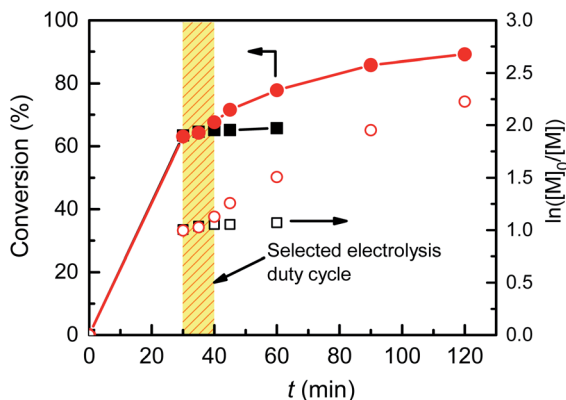
Fig. 3 Determination of the duty cycle by following the evolution of conversion and \ln([M]_0/[M]) vs. t for eATRP of 50 vol% nBA in DMF+0.1 M Et_4NBF_4 at T = 45^\circ C , performed in an undivided cell with a Pt (squares) or a Cu (circles) cathode at E_{app} = E_{1/2} - 0.06 V and a sacrificial Al anode. Electrolysis was switched off on both electrodes after 30 minutes. Conditions: nBA/EBiB/Cu(OTf)_2/Me_6TREN/Et_4NBr = 349/1/0.1/0.3/0.1 , C_{nBA} = 3.49 M.
