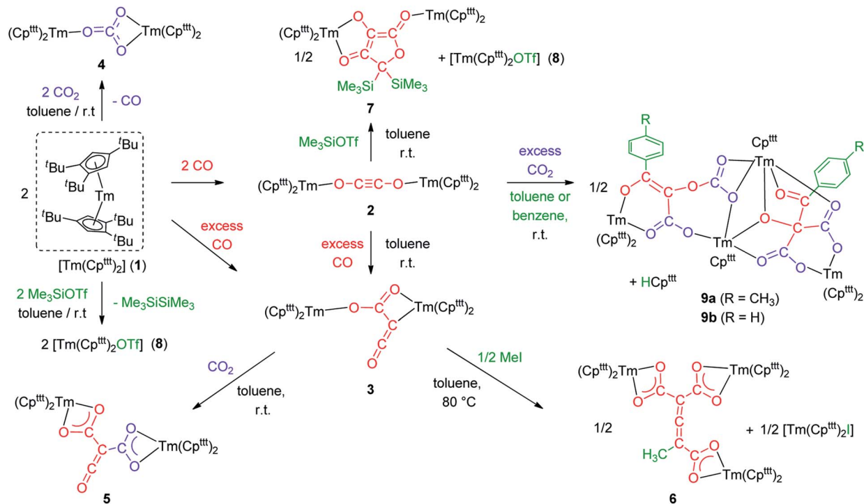
Scheme 5 Summary scheme of all the reactivity described in this study starting from [Tm(Cp^{*tt})_2] (1).
