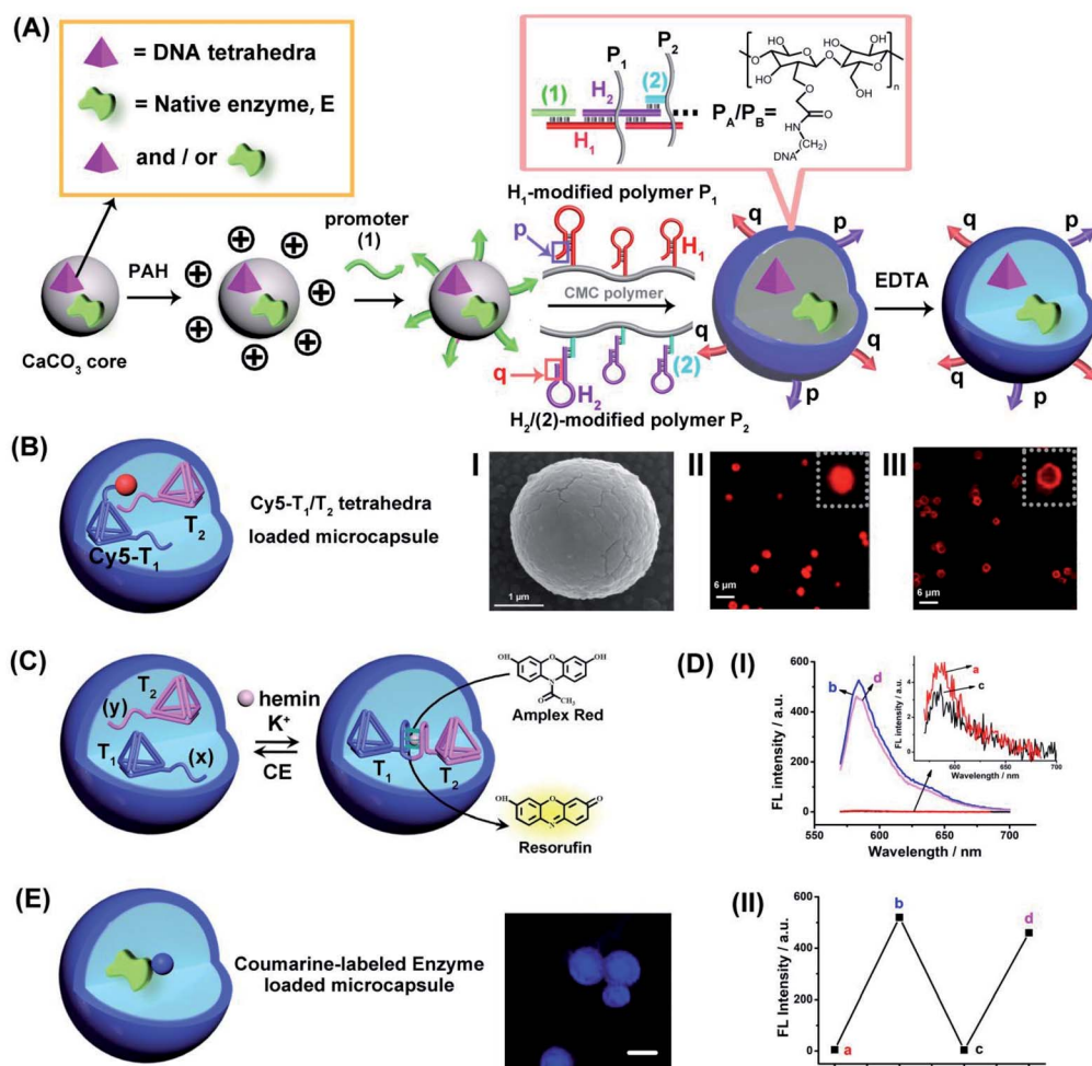
Fig. 1 (A) Schematic preparation of DNA tetrahedra and/or native enzyme-loaded carboxymethyl cellulose (CMC) DNA duplex-crosslinked hydrogel microcapsules. (B) Schematic composition of Cy5-labeled tetrahedra T 1 /T 2 -loaded microcapsules. Panel I-SEM image of the hydrogel-coated \text{CaCO}_3 microparticles loaded with the Cy5-T 1 /T 2 DNA tetrahedra. Scale bar = 1 \mu\text{m} . Panel II-Confocal fluorescence microscopy image of the hydrogel-coated \text{CaCO}_3 microcapsules loaded with Cy5-labeled T 1 and T 2 . Scale bar = 6 \mu\text{m} . Panel III-Confocal fluorescence microscopy image of the hydrogel-stabilized microcapsules loaded with Cy5-labeled T 1 and T 2 after etching of the \text{CaCO}_3 core. Scale bar: 6 \mu\text{m} . (C) Cyclic K + -ions stimulated dimerization of the DNA tetrahedra T 1 /T 2 by hemin/G-quadruplex DNAzyme bridges and their separation by means of 18-crown-6-ether (CE). Formation of the hemin/G-quadruplex is probed by the DNAzyme catalyzed oxidation of Amplex Red to the fluorescent Resorufin. (D) Panel I-Fluorescence spectra of the bulk solution that includes Amplex Red, 0.083 mM, hemin, 0.167 \mu\text{M} and H 2 O 2 , 4.16 mM upon: (a) Without K + -ions. (b) and (d) Cyclic addition of K + -ions, 50 mM. (c) Intermediate addition of 200 mM CE. Panel II-Switchable fluorescence intensities of microcapsule stimulated generation of Resorufin. (E) Schematic composition of Coumarin-labeled GOx-loaded microcapsules and confocal fluorescence microscopy image of the Coumarin-labeled GOx-loaded microcapsules. Scale bar = 2 \mu\text{m} .
