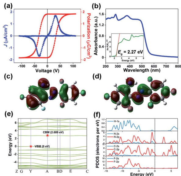
Fig. 4 (a) P - E hysteresis loops of the APFA thin film via a double-wave method at room temperature. (b) UV-vis absorption spectra of APFA. Inset: the Tauc plot for APFA. (c) HOMO and (d) LUMO of the APFA molecule. (e) The calculated band structure of APFA and (f) the corresponding PDOS.
