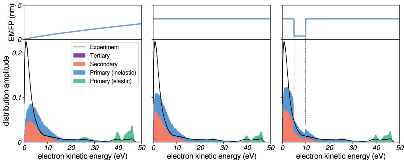
Fig. 5 Influence of the EMFP. Comparison of simulated spectra to experimental results, for a photon energy corresponding to harmonic 37 of \approx 800 nm ( \approx 57.6 eV), for several choices of EMFP. Left: EMFP extrapolated from reported results (Fig. 3a). Middle: constant 3 nm EMFP. Right: constant EMFP with a local square-shaped minimum.
