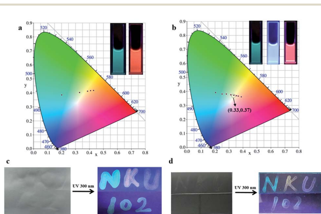
Fig. 5 The CIE chromaticity diagrams of the photoluminescence color changes from varying the ratios of (a) RhB (inset: photographs of HABr/CB[8]/LP and HABr/CB[8]/LP/RhB) and (b) SR101 (inset: photographs of HABr/CB[8]/LP, HABr/CB[8]/LP/0.005SR101 and HABr/CB[8]/LP/SR101). The photoluminescence inks based on the light harvesting system: (c) photographs writing "N" with HABr/CB[8]/LP, "K" with HABr/CB[8]/LP/RhB, "U" with HABr/CB[8]/LP/SR101 and "102" with HABr/CB[8]/LP/0.005SR101 (c) on filter paper under natural light and under UV light; (d) doped PVA on glass under natural light and under UV light.
