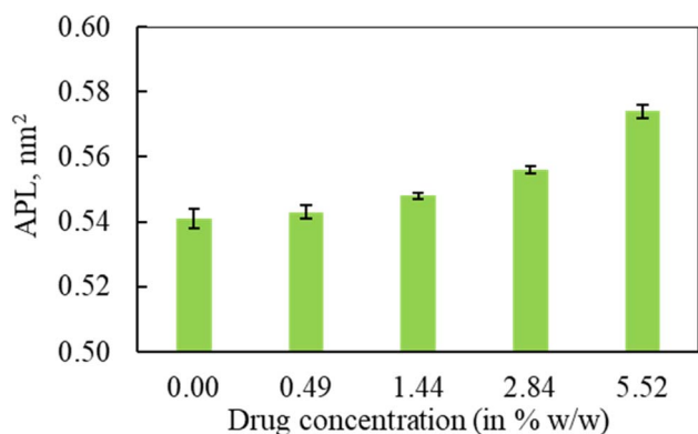
Fig. 6 The effect of hydrocortisone concentration on the area per lipid (APL) from the simulation of protein containing system at 20 \text{ mN m}^{-1} . The data were estimated over the last 1 \mu\text{s} of the 2 \mu\text{s} simulation. The error bar refers to standard deviations of the APL data across the frames.
