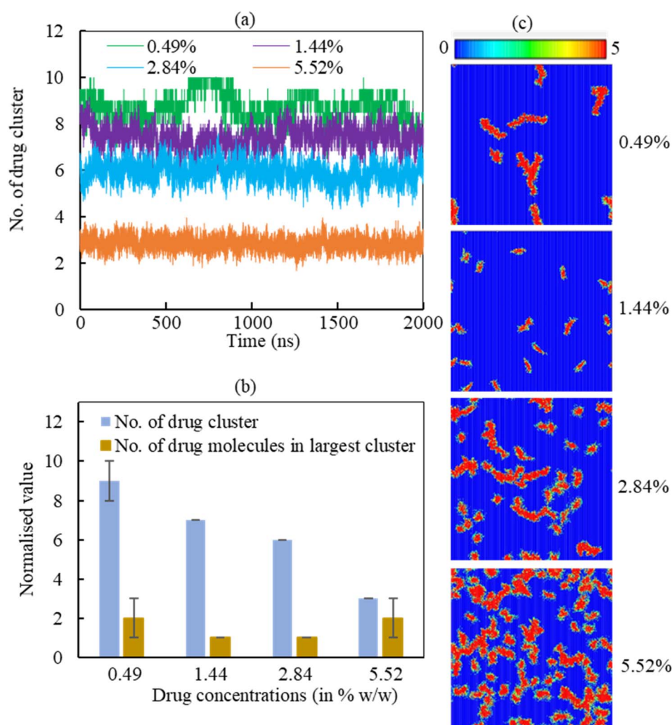
Fig. 9 Normalised hydrocortisone cluster analysis of four drug concentrations (0.49, 1.44, 2.84, 5.52% w/w) in the LSM at surface tension \gamma = 20 mN m ^{-1} . (a) Number of normalised hydrocortisone cluster formation over the time. (b) Number of normalised hydrocortisone cluster and the number of hydrocortisone molecules in the largest cluster are shown for different hydrocortisone concentrations. (c) The two-dimensional (2D) density map of the hydrocortisone to show the cluster formation on the monolayer at different hydrocortisone concentrations. The data was normalised using the number of drugs in the corresponding drug concentration with respect to the 0.49% w/w hydrocortisone concentration.
