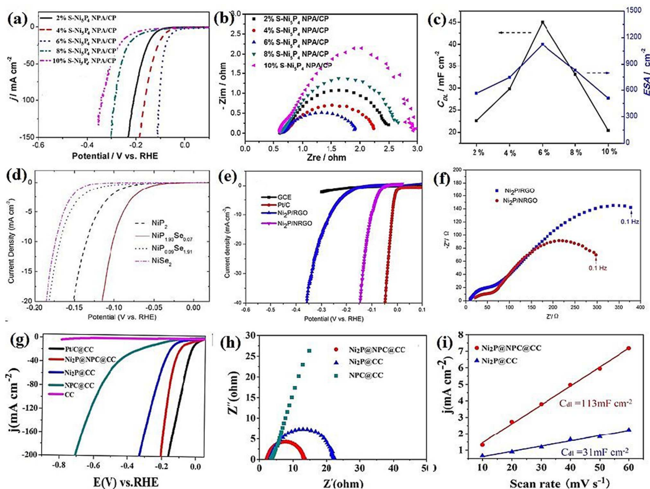
Fig. 15 Sulfur-doped Ni 5 P 4 : (a) LSV curves in 0.5 M H 2 SO 4 , (b) EIS plots and (c) ECSA as a function of sulfur content (reproduced from ref. 120 with permission from the America Chemistry Society, Copyright 2018). (d) LSV curves of selenium-doped NiP 2 (reproduced from ref. 121 with permission from the America Chemistry Society, Copyright 2015). Nickel phosphide nanoparticle–nitrogen-doped graphene hybrid: (e) LSV curves and (f) EIS plots (reproduced from ref. 77 with permission from Elsevier, copyright 2015). Nickel phosphide nanoparticles with nitrogen and phosphorus co-doped porous carbon: (g) LSV curves, (h) EIS plots and (i) electrochemical double-layer capacitance (reproduced from ref. 123 with permission from Elsevier, copyright 2020).
