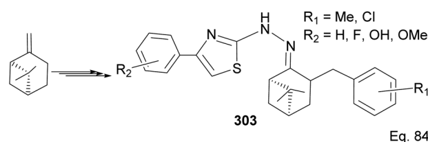
Scheme 78 Synthesis of (–)-β-pinene-based thiazole.
