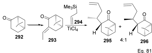
Scheme 75 TiCl 4 -mediated synthesis of allylic nopinone enantiomer 295 and 296 (precursors in the preparation of (+)-nootkatone and its derivatives).
