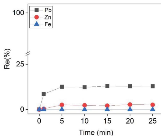
Fig. 7 Effect of ion flotation time on the recovery efficiency of Zn, Pb and Fe from the PLS after the cementation step. Conditions: [\text{CTAB}] = 0.9 \text{ mmol L}^{-1} , [\text{Zn}]_i = 22.5 \text{ mmol L}^{-1} , [\text{Pb}]_i = 3.5 \text{ mmol L}^{-1} , [\text{Fe}]_i = 500 \text{ mmol L}^{-1} , [\text{EtOH}] = 0.5\% (v/v), V = 50 \text{ mL} , flowrate = 25 \text{ mL min}^{-1} .
