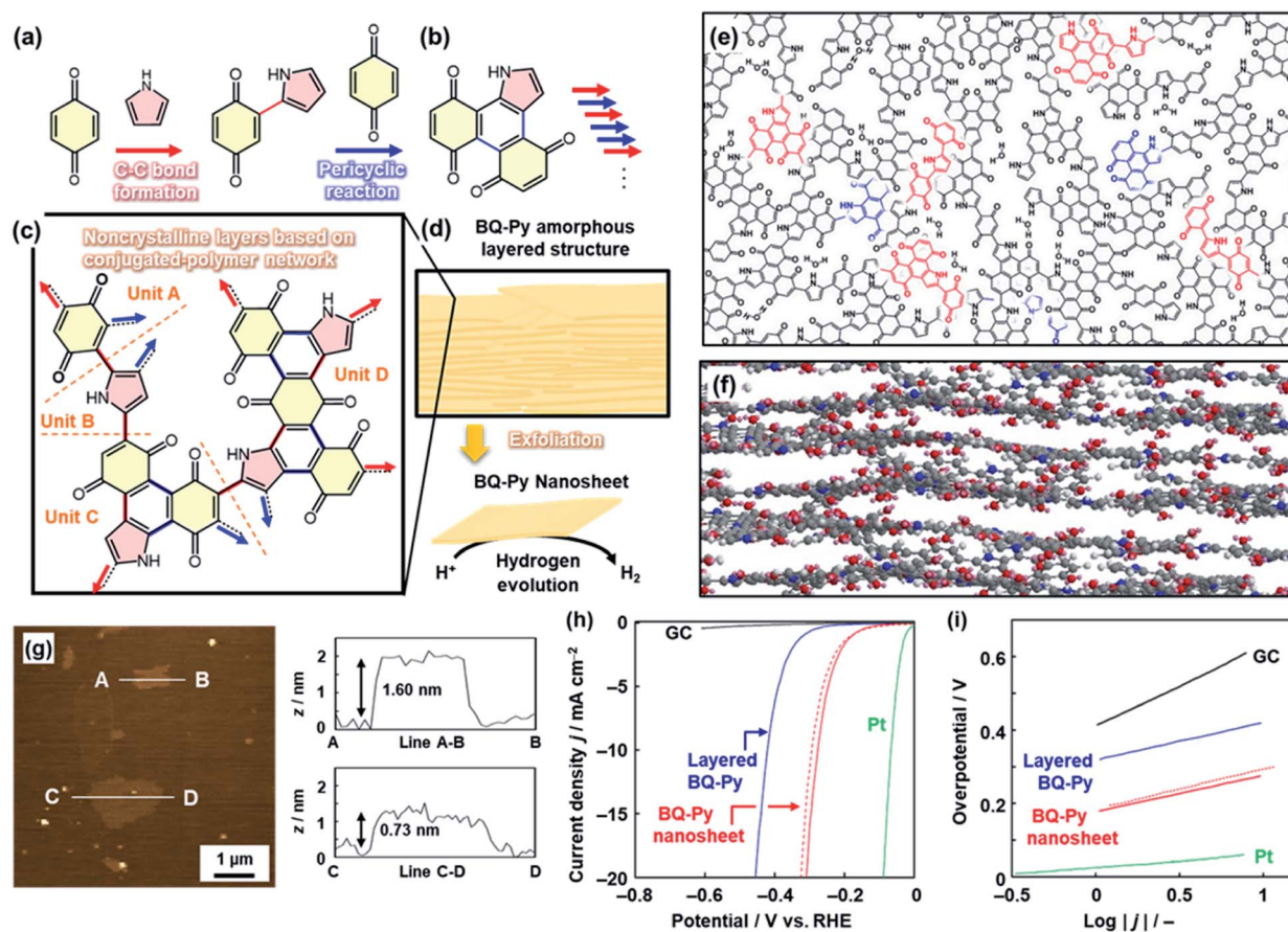
Fig. 6 Copolymerization of the heteroaromatic monomer inside of the crystals. (a and b) Successive C–C bond formation (red arrow) and the pericyclic reaction between BQ and Py (blue arrow). (c) Four structure units of the BQ–Py polymer in the noncrystalline layers. (d) Amorphous layered structure and its exfoliation into the nanosheets with enhanced catalytic properties for the electrochemical HER. (e and f) Schematic models of top (e) and side (f) views of the layered BQ–Py. The upper and lower layers are grown from the red and blue parts in the panel (e), respectively. (g) AFM images and their height profiles. (h and i) LSV curves (h) and Tafel slopes (i) of the bare GC electrode (black line), the layered BQ–Py (blue line), the BQ–Py nanosheets (red line), and the BQ–Py nanosheets after cyclic voltammetry in the range 0 to -0.3 V (vs. RHE) for 500 cycles (red dashed line). Reproduced from ref. 24 with permission from the Springer Nature.
