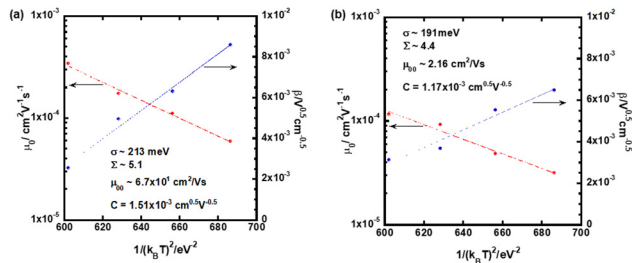
Fig. 5 Plots of zero-field mobility \mu_0 and field-dependence of the hole mobility \beta as a function of the square of 1/k_B T in the N* phase of (a) compound 1 and (b) compound 2 .
