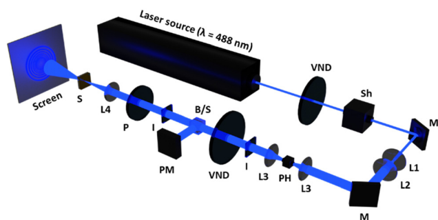
Fig. 2 Schematic diagram of the optical setup for self-diffraction measurements. VND, variable neutral density filter; Sh, shutter; M, mirror; L1, plane concave lens ( f = -8\text{ cm} ); L2, plane convex lens ( f = 20\text{ cm} ); L3, plane convex lens ( f = 7.5\text{ cm} ); PH, pinhole; I, iris; PM, power meter; B/S, beam splitter; P, polarizer; L4, bi-convex lens ( f = 15\text{ cm} ); S, LC cell sample. The beam diameter before L4 was 1.9 mm. The sample was placed at a focal point of L4 where the diameter of the beam was 50 \mu\text{m} .
