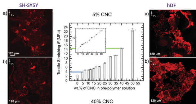
Fig. 3 Middle: Evolution of the tensile Young's modulus of 6A-PCL/CNC composite films with the addition of CNCs (data measured by tensile stretching). The values in blue and green noted tensile deformation values of brain and skin tissues, respectively. The inset shows the E in log10 scale, to emphasize the exponential dependency found with the addition of CNCs. Right and left confocal images of SH-SY5Y and hDF (respectively) cells seeded into (a) 5 wt% and (b) 40 wt% 6A-PCL/CNC composite foams after two weeks of proliferation. Adapted from ref. 82, Royal Society of Chemistry.
