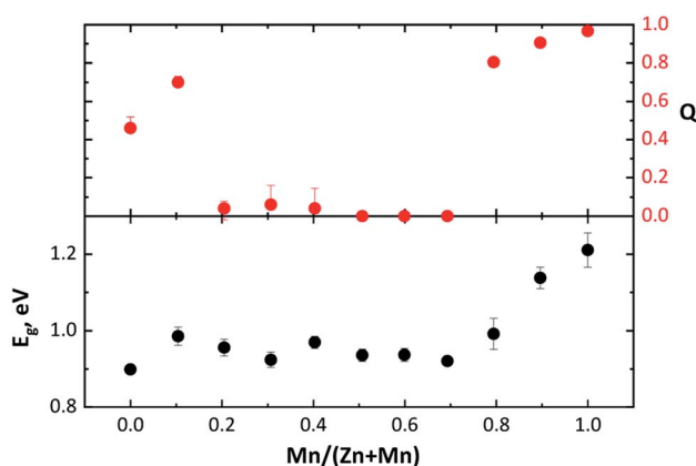
Fig. 9 Band gap energy E_g and order parameter Q of \text{Cu}_2(\text{Zn}_{1-x}\text{Mn}_x)\text{SnSe}_4 mixed crystals dependent on the Mn/(Mn + Zn) ratio.
