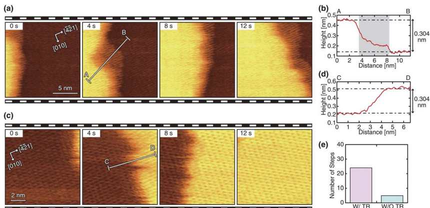
Fig. 3 (a and c) Successive HS-FM-AFM images of the growing calcite step edges with a complex non-linear shape obtained on the calcite (10 \bar{1} 4) surface in the supersaturated solution. (a) With a TR. \Delta f = 2.2 kHz. A = 0.45 nm. 2 s per frame. 500 \times 500 pix ^2 . (c) Without a TR. \Delta f = 1.7 kHz. A = 0.14 nm. 2 s per frame. 500 \times 500 pix ^2 . (b and d) Height profiles measured along the lines A–B and C–D. (e) Number of complex steps with and without a TR observed in this study.
