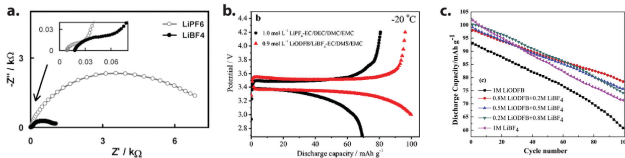
Fig. 14 (a) Impedance spectra at -20\text{ }^\circ\text{C} of fully-charged Li-ion cells containing 1 molal \text{LiPF}_6 in EC/DMC/DEC 1:1:1 w/w, compared to 1 molal \text{LiBF}_4 in the same solvent mixture. Charge-transfer resistance is significantly reduced in the \text{LiBF}_4 -based electrolyte. Reprinted by permission from Springer Nature: ref. 123, copyright 2002. (b) Initial -20\text{ }^\circ\text{C} charge/discharge curves of \text{Li}||\text{LiFePO}_4 cells with a mixed \text{LiDFOB/LiBF}_4 electrolyte versus a standard mixture. The discharge rate is 0.5C. Reprinted by permission from Springer Nature: ref. 77, copyright 2014. (c) Cycling performance of \text{Gr}||\text{LiNi}_{0.5}\text{Mn}_{1.5}\text{O}_4 cells at -20\text{ }^\circ\text{C} in electrolytes containing varying ratios of \text{LiDFOB} to \text{LiBF}_4 , with 1 M total salt in EC/DMC/EMC 1:1:1 w/w. A combination of 0.8 M \text{LiDFOB} and 0.2 M \text{LiBF}_4 strikes the best balance between initial capacity and retention. Reprinted from ref. 129 with permission from Elsevier.
