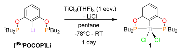
Scheme 2 Synthesis of 1.
