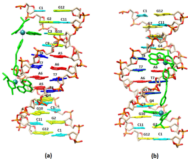
Fig. 8 Cartoon representation of the binding of (5) to the DNA sequence d(5'-\text{CGCGTAGGCC}-3') 2 based on NMR data. (a) –C3G4– major groove binding extended towards G12, (b) –G10C9– major groove binding extended towards C1.
