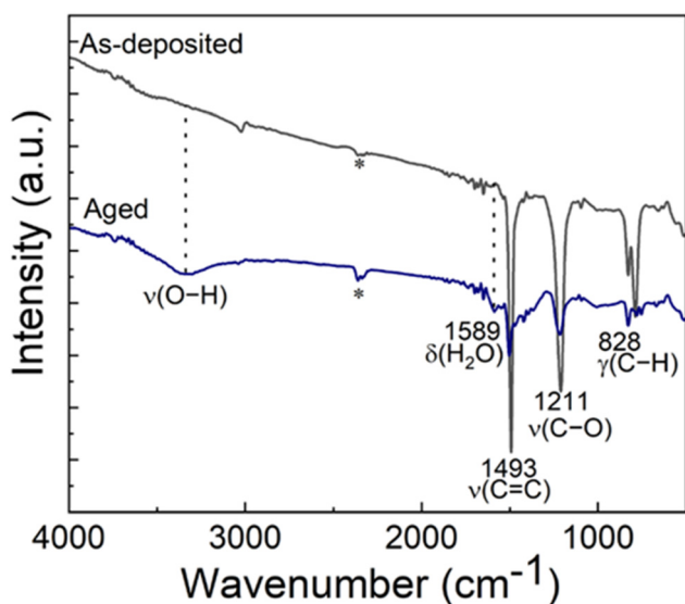
Fig. 6 Stability studies of the Zn-HQ thin films deposited at 60 °C on Si(100) in this study. Comparison of FTIR spectrum of a 95 nm thick Zn-HQ thin film immediately after the deposition and after two weeks in ambient conditions. The bands marked with * are caused by adsorbed \text{CO}_2 .
