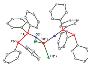
Fig. 5 Molecular structure of [\text{FeCl}_2(\text{PPO})_2] ( 1 ). Co-crystallised solvent molecules atoms are omitted for clarity. Selected bond lengths ( \text{\AA} ) and angles ( ^\circ ): Fe(1)–O(1) 2.017(2) , Fe(1)–O(2) 2.006(3) , Fe(1)–Cl(1) 2.264(1) , Fe(1)–Cl(2) 2.276(1) , P(1)–O(1) 1.506(3) , P(1)–P(2) 2.202(1) , P(3)–O(2) 1.493(3) , P(3)–P(4) 2.188(1) , O(1)–Fe(1)–O(2) 97.9(1) , Cl(1)–Fe(1)–Cl(2) 114.90(4) , O(1)–P(1)–P(2) 117.3(1) , O(2)–P(3)–P(4) 117.8(1) .
