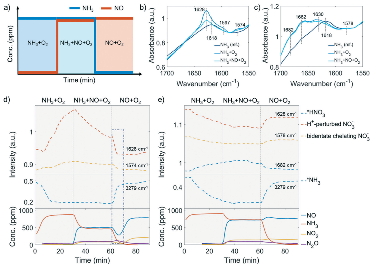
Fig. 6 a) Procedure of the operando diffuse reflectance Fourier transform spectroscopy (DRIFTS) experiment performed. The experiment was conducted after \text{O}_2 calcination at 550^\circ\text{C} followed by \text{NH}_3 + \text{O}_2 , \text{NH}_3 + \text{NO} + \text{O}_2 and \text{NO} + \text{O}_2 reaction at 250^\circ\text{C} with 1000 ppm of \text{NH}_3 and/or 1000 ppm \text{NO} balanced by 5% \text{O}_2/\text{He} . The obtained operando DRIFTS spectra of surface nitrates in b) fresh and c) 850^\circ\text{C} steamed zeolite ZSM-5. The evolution of selective bands representing surface nitrates (upper panel) and adsorbed \text{NH}_3 (middle panel) were followed and the recorded concentration of effluent gas composition (bottom panel) in the d) fresh and e) 850^\circ\text{C} steamed zeolite Cu-ZSM-5. Missing datapoints at the beginning of the experiment (Fig. 6d and e, bottom panel) are due to values below the limit of detection.
