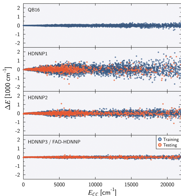
Fig. 2 Energy difference \Delta E = E_{\text{CC}} - E_{\text{PES}} as a function of the reference energy E_{\text{CC}} relative to the energy of the global minimum for the QB16 PES, 55 HDNNP1, HDNNP2, and HDNNP3 (=FAD-HDNNP). The root-mean-squared errors (RMSE) for the HDNNPs are provided in Table 1.
