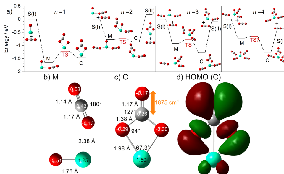
Fig. 6 (a) Potential energy surfaces for \text{HoO}(\text{CO}_2)_n^+ ( n=1\text{--}4 ) generated at the UB3P86/Def2-TZVP level of theory showing the relative energies of \text{Ho}(\text{CO}_3)(\text{CO}_2)_{n-1}^+ (labelled C-isomers) and \text{HoO}(\text{CO}_2)_n^+ (M-isomer) structures. The surfaces show the transformation between species. S(i) represents the \text{HoO}(\text{CO}_2)_{n-1}^+ isomer and free \text{CO}_2 and S(ii) represents the \text{Ho}(\text{CO}_3)(\text{CO}_2)_{n-2}^+ isomer with free \text{CO}_2 . (b and c) structural details and (Hirshfeld) partial charges of the M and C isomers, respectively for the n=1 case and (d) the C isomer HOMO.
