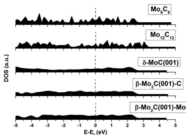
Fig. 4 Density of states (DOS) for the bare carbide nanoparticles and surfaces. The β-Mo 2 C(001) surface has C- and Mo-terminations, hence, both surfaces are included. Mo 6 C 6 and Mo 12 C 12 were taken as representative nanoparticles.
