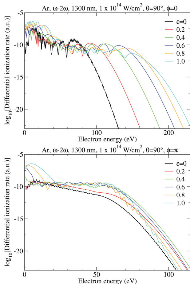
Fig. 7 The logarithm of the differential ionization rate of Ar atoms as a function of the photoelectron energy in electron volts for ionization by an \omega - 2\omega BEOTC field with the ellipticities \varepsilon = \varepsilon_1 = \varepsilon_2 denoted in the panels. Both the direct and the rescattered electrons are included. The intensities of the field components are I_1 = I_2 = 1 \times 10^{14} \text{ W cm}^{-2} , the fundamental wavelength is 1300 nm, and emission is in the direction of the semi-minor axis of the polarization ellipse ( y axis). The relative phase is \phi = 0 (upper panel) and \phi = \pi (lower panel).
