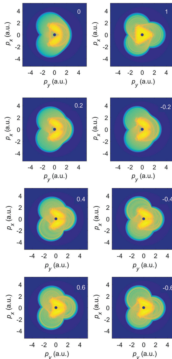
Fig. 8 The logarithm of the differential ionization rate (in a.u.) of Ar atoms, presented in false colors in the photoelectron momentum plane, for ionization by an \omega - 2\omega BEOTC field with the ellipticity \varepsilon = \varepsilon_1 = \varepsilon_2 denoted in the upper right corner of each panel, and with the relative phase \phi = 0 . Both the direct and the rescattered electrons are included. The false-color scale covers 13 orders of magnitude (the logarithm of the rate extends from -6 down to -19 ). The other laser parameters are as in Fig. 7.
